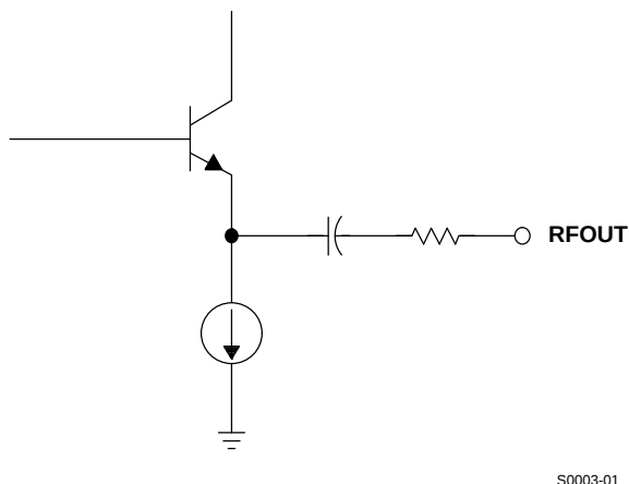
Figure 51. RFOUT Equivalent Circuit
